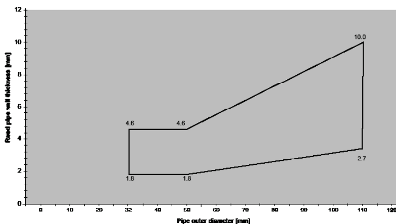
Application area PP pipes with pipe end configuration UU
