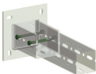
Art. 8650335 Connettore per profilo quadro Front connection for heavy rail profile
